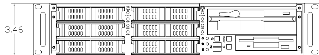
FRONT VIEW - DOOR OPEN
