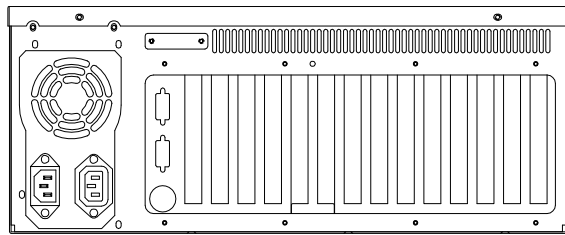
REAR VIEW - PS/2 POWER
