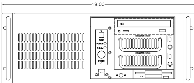
FRONT VIEW - DOOR OPEN
